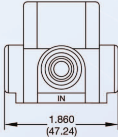
1/8-27 NPT PORTING
