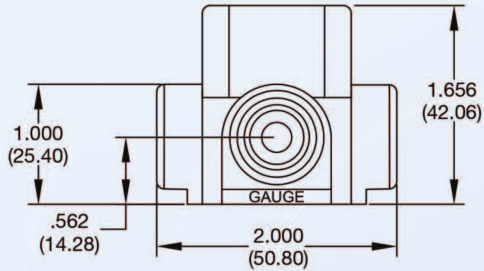
1/4-18 NPT PORTING
